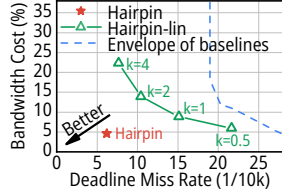
Figure 24: Heuristic-based Hairpin (Hairpin-lin). The envelope of baselines is from Figure 10(b).
