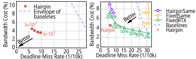
Figure 13: Parameter sensitivity of \lambda in the utility function of Hairpin.
