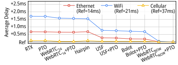
Figure 21: Average end-to-end delay of in the experiments in §4.3. We trim the lowest average delay in different traces for comparison.
