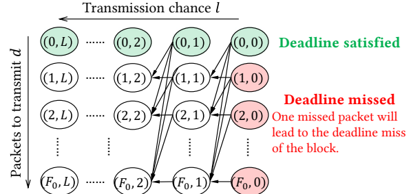
Figure 8: The absorbing Markov chain in redundancy rate optimization at given loss rate and frame size. l is the estimated remaining transmission chances for the packets to transmit.
