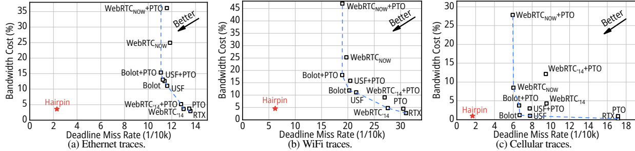
Figure 10: Trace-driven simulation. The blue dashed line is the envelope of all baselines on the Pareto frontier.
