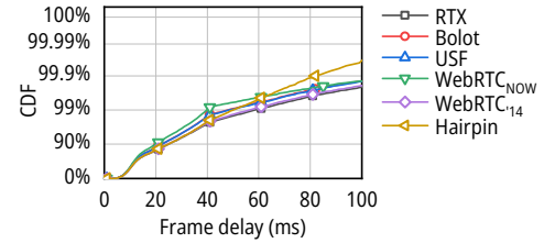
Figure 22: The distribution of the delivery time of each frame. Note that the y-axis is log-scaled.
