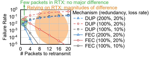
Figure 9: A theoretical illustration of the failure rate of retransmitting different numbers of packets by per-packet duplication or constructing FEC blocks. The failure rate of DUP increases with the number of packets to retransmit, since we need to ensure every data packet is delivered. We vary the redundancy rate and loss rate.
